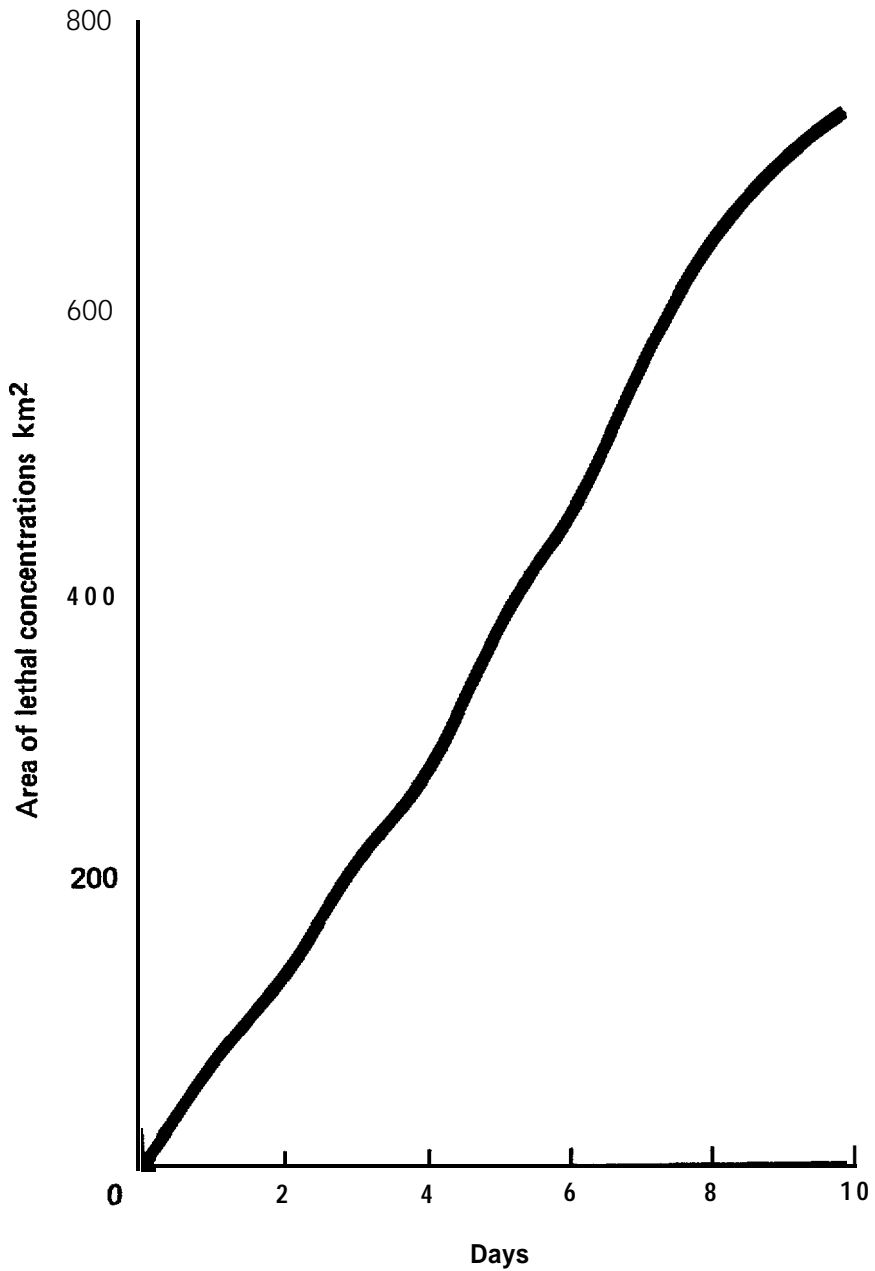
Figure 15.--Areal coverage of concentrations of fuel oil lethal to sockeye salmon after 24 hrs (>0.45 ppm) resulting from a simulated spill of 240,000 bbl of No. 2 diesel oil off Port Heiden or Port Moller in Bristol Bay. (Data from Rand Corporation.)
