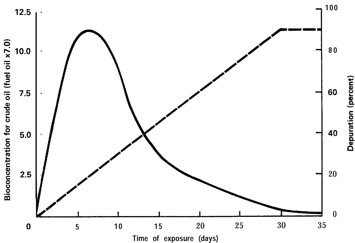
Figure 11 --- Functions describing the bioconcentration and depuration of crude oil in the tissues of salmon exposed to a naturally weathering oil spill. (Bioconcentration factors for No. 2 diesel oil are 7 times higher than those for crude oil.)
