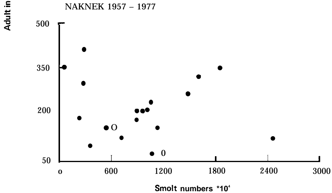
Figure 5.--Returns of adult Bristol Bay sockeye salmon and their estimated numbers (or index) as smelts outmigrating from the rivers. (Data sources detailed in text.)
