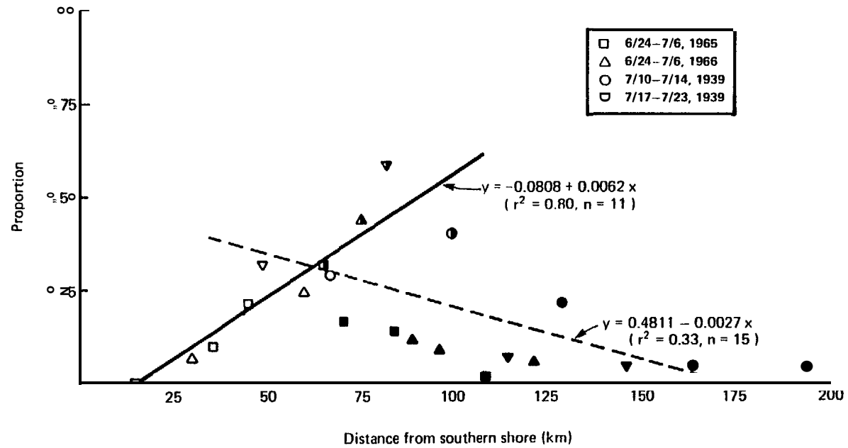
Figure 4. --Proportions of total sockeye salmon caught in exploratory gill net surveys in Bristol Bay, that were caught at varying distances from shore. Data from Straty (1975).
