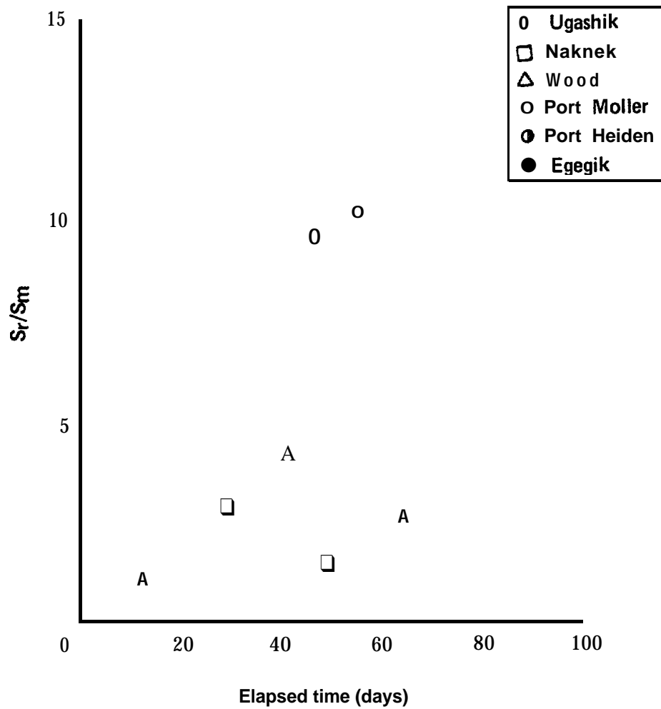
Figure h---Ratio of standard deviation of recaptures to standard deviation of releases for marked juvenile sockeye salmon released into rivers leading to Bristol Bay. (Data from Straty 1974. Symbols denote river of release; shading point of recapture.)
