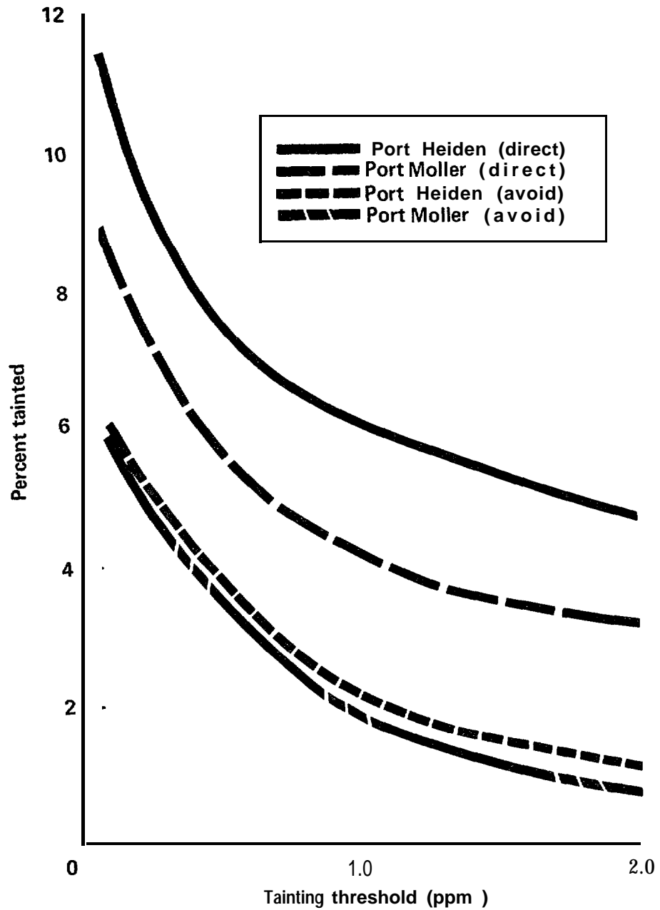
Figure 19--- Percentages of adult sockeye salmon migrating through the fuel oil spill grids that would be tainted at different tainting thresholds and under the assumptions of avoidance or direct migration.
