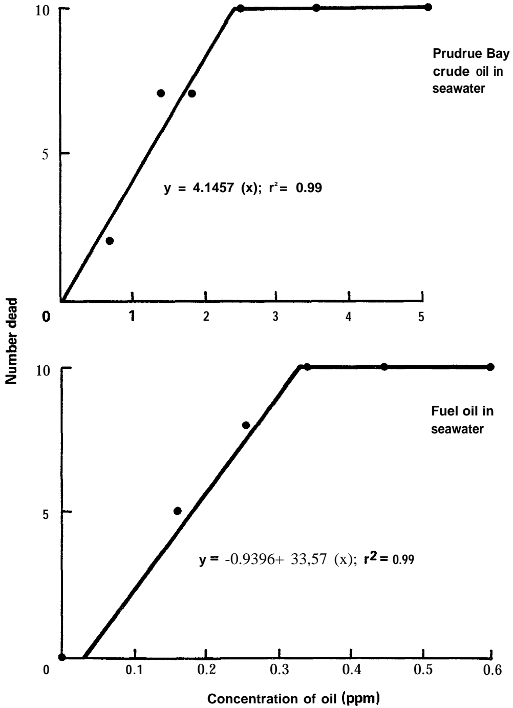
Figure 6.--Number of sockeye salmon smelts dying (out of 10) following exposure to oil in static seawater tests for 96 hr. Data from Adam Moles (NOAA).
