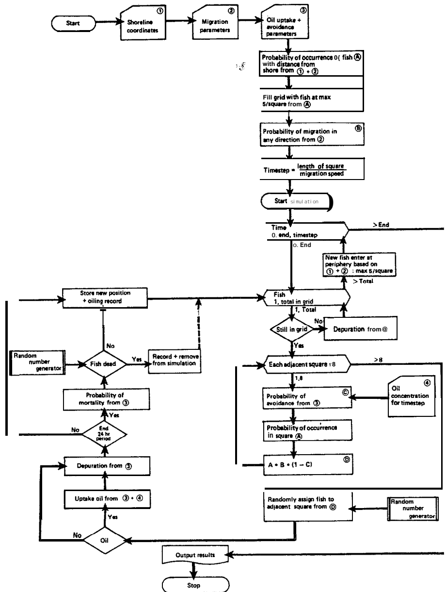
Figure 3---Flow chart of processes involved in simulating the movement of sockeye salmon through an oil spill in Bristol Bay.
